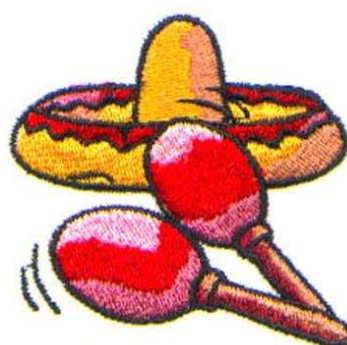
Mexican Hat File: LA0231 Size: 2.24" W X 2.17" H
